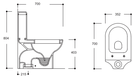
K001KLZ00 COMPACT KLOZET (ALT ÇIKIŞLI) K001RZV REZERVUAR K002KLZ00 COMPACT CLOSET (S-TRAP) K001RZV CISTERN
