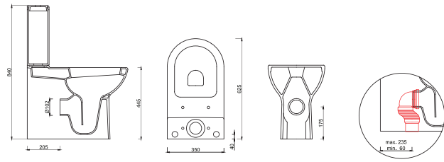
K032KLZ00 COMPACT ENGELLİ DUVARA DAYALI KLOZET K001RZV REZERVUAR K033KLZ00 COMPACT UNIVERSAL COMFORT HEIGHT BACK TO WALL CLOSET K001RZV CISTERN
