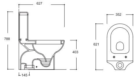
K007KLZ00 COMPACT KLOZET (ALT ÇIKIŞLI, KISA Q) K001RZV REZERVUAR K008KLZ00 COMPACT CLOSET (S-TRAP, SHORT Q) K001RZV CISTERN
