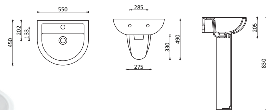
K004LVB01 COMPACT LAVABO (45x55) K001AYK00 KOLON AYAK CA02AYK00 YARIM AYAK
