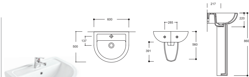
K005LVB01 COMPACT LAVABO (50x60) K001AYK00 KOLON AYAK KU02AYK00 YARIM AYAK
